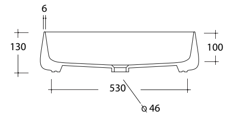
Art. PAD4B60001
