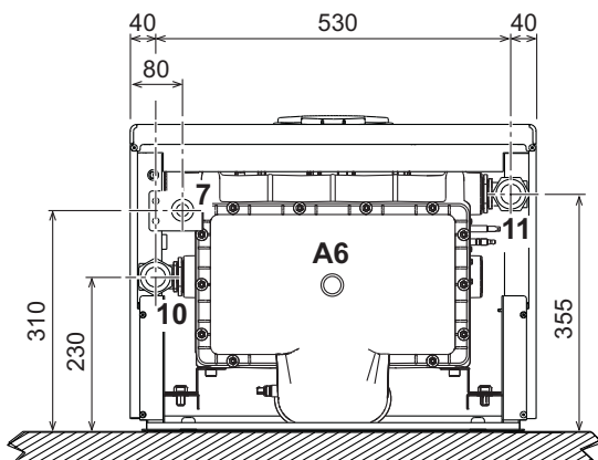
fig. 67- Bottom view - model FORCE W 150
