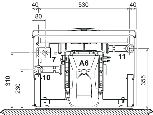
fig. 65- Vista inferior mods. FORCE W 60 y FORCE W 80
