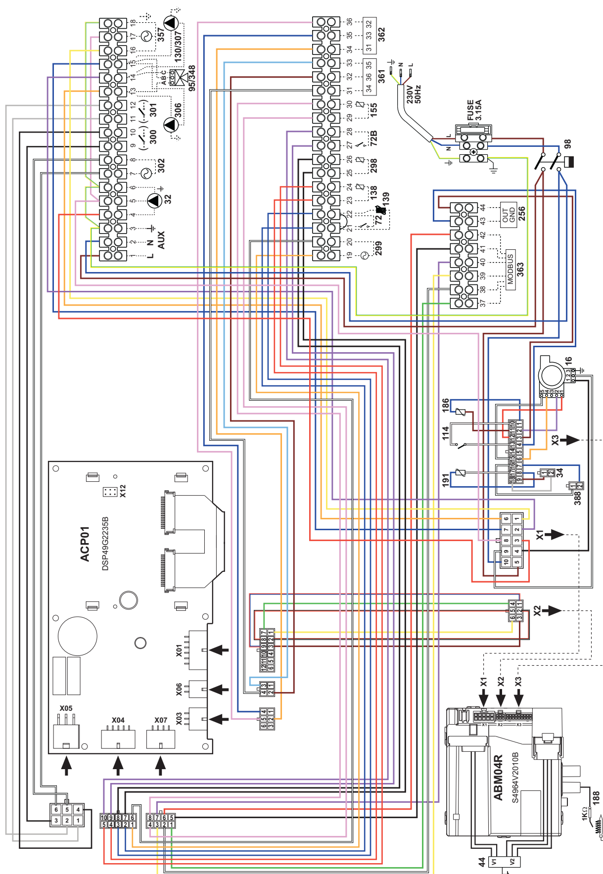
fig. 75- Wiring diagram - models FORCE W 99, FORCE W 120 and FORCE W 150
