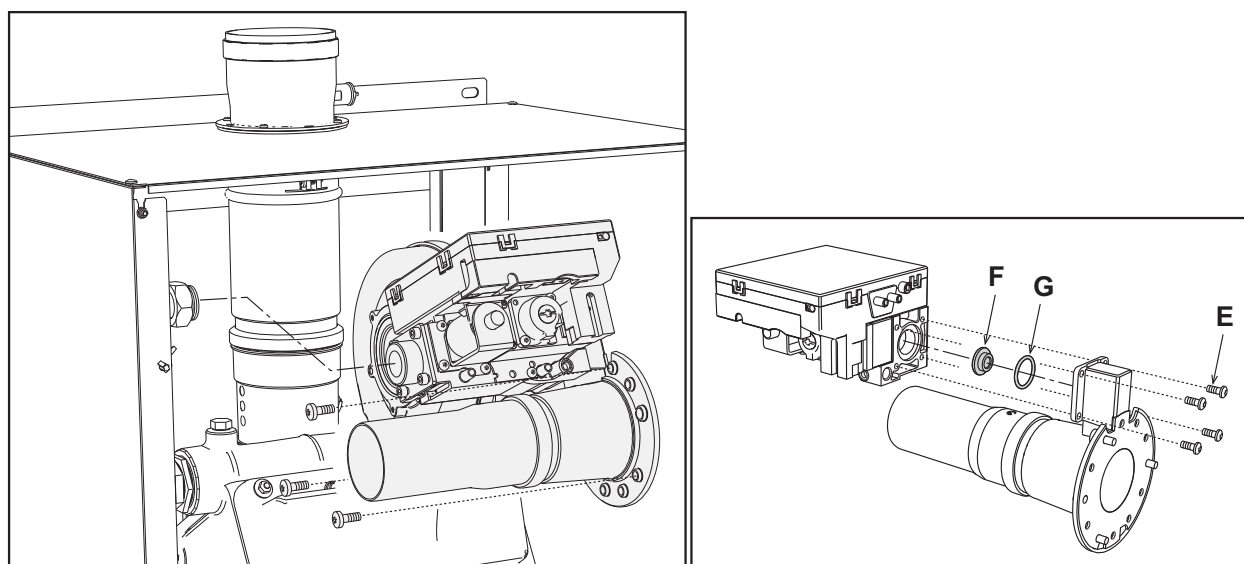
fig. 58- Models FORCE W 99, FORCE W 120 and FORCE W 150
