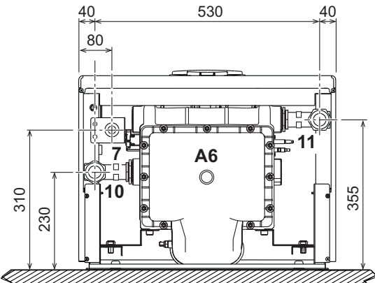
fig. 66- Vista inferior mods. FORCE W 99 y FORCE W 120
