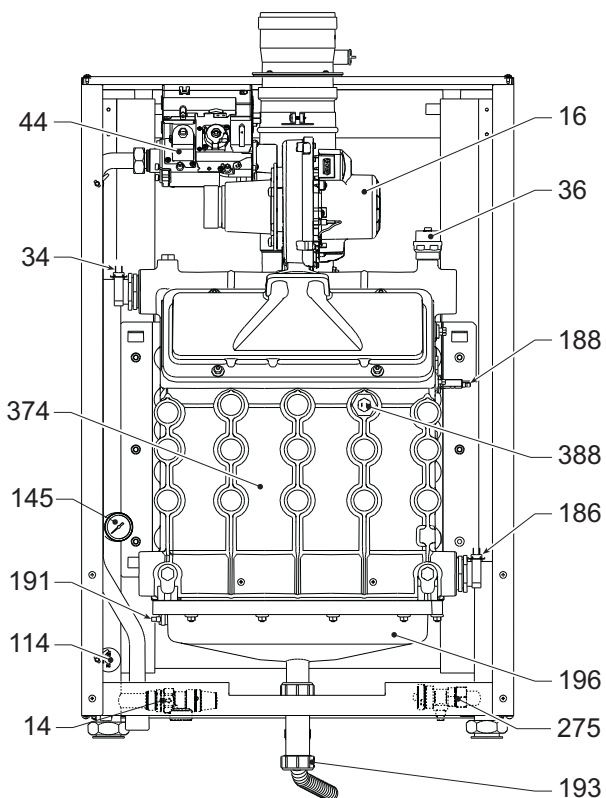
fig. 70- General view - model FORCE W 150
