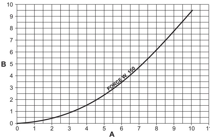
fig. 73- Pressure loss diagram - models FORCE W 150
