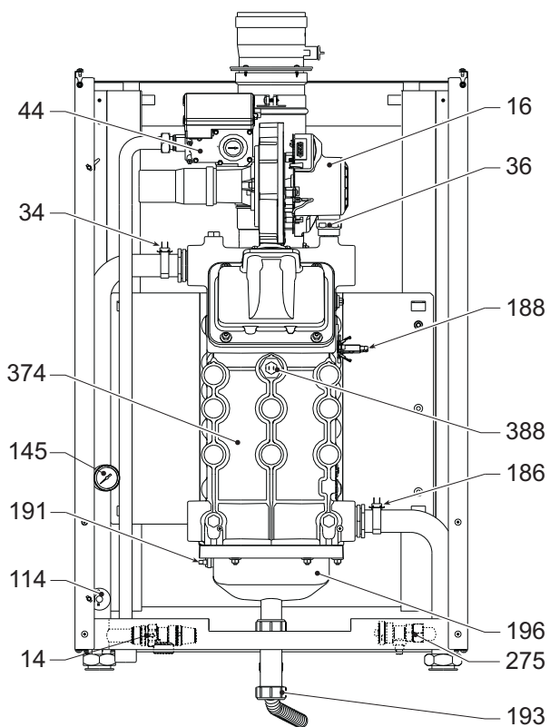
fig. 68- General view - model FORCE W 60 and FORCE W 80
