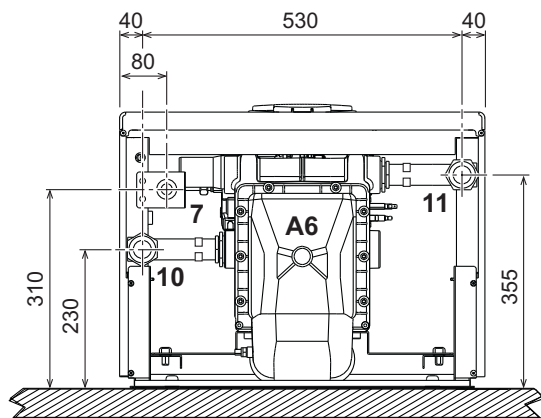
fig. 65- Bottom view - model FORCE W 60 and FORCE W 80
