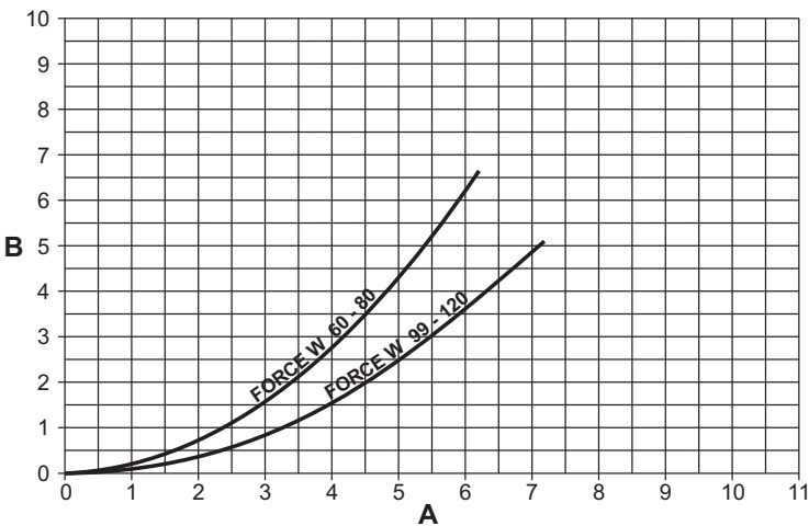
fig. 72- Pressure loss diagram - models FORCE W 60 - FORCE W 80 - FORCE W 99 - FORCE W 120
