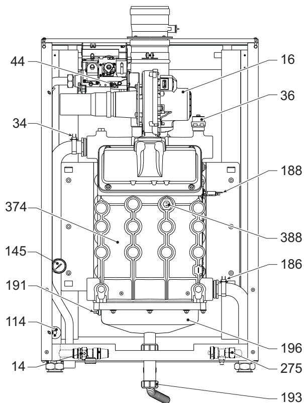
fig. 69- Vista general mods. FORCE W 99 y FORCE W 120
