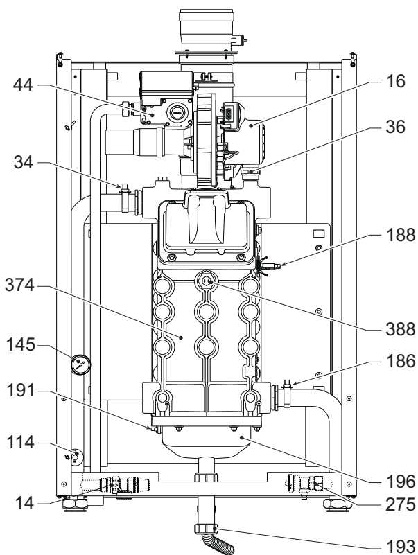
fig. 68- Vista general mods. FORCE W 60 y FORCE W 80
