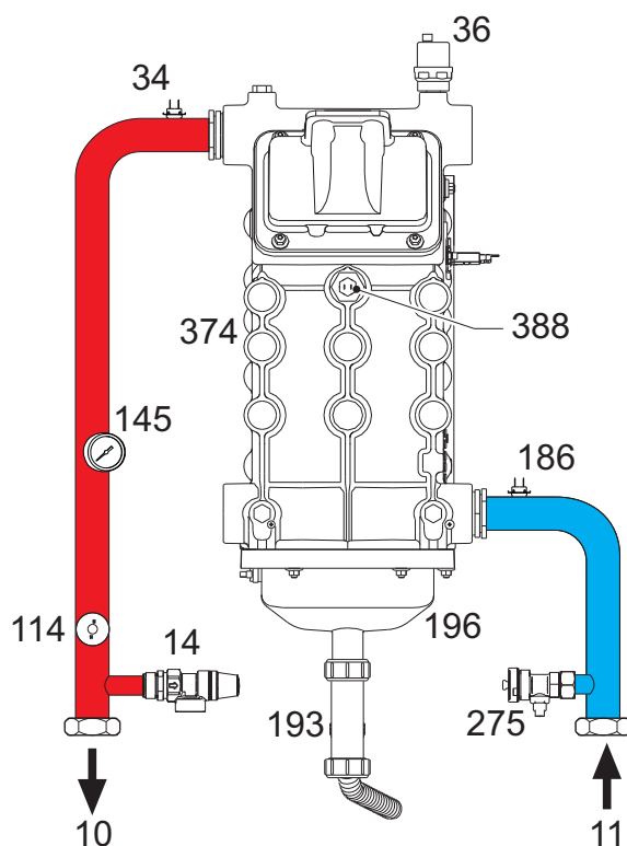
fig. 71- Hydraulic circuit
