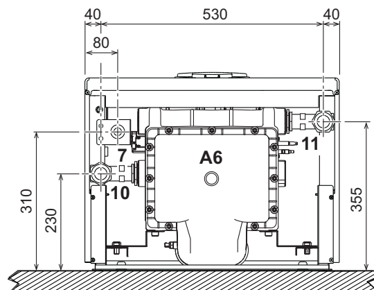
fig. 66- Bottom view - model FORCE W 99 and FORCE W 120
