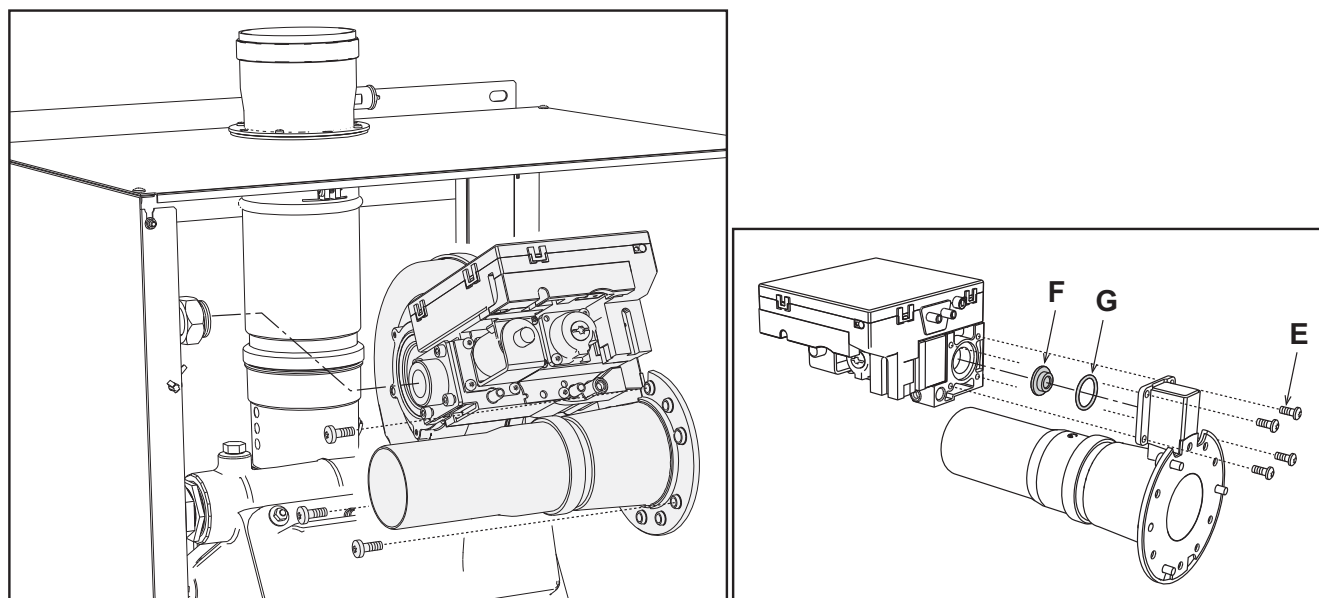
fig. 58 - Modelli FORCE W 99, FORCE W 120 e FORCE W 150
