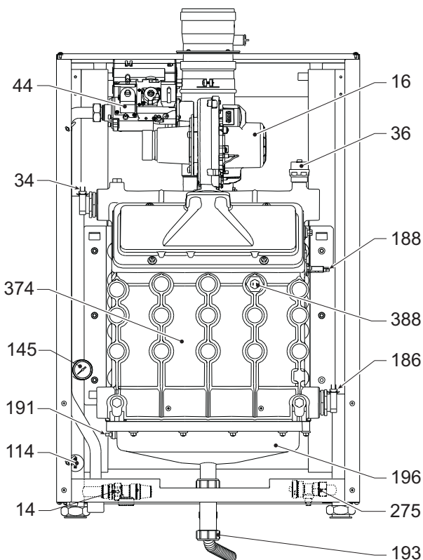
fig. 70- Vista general mod. FORCE W 150
