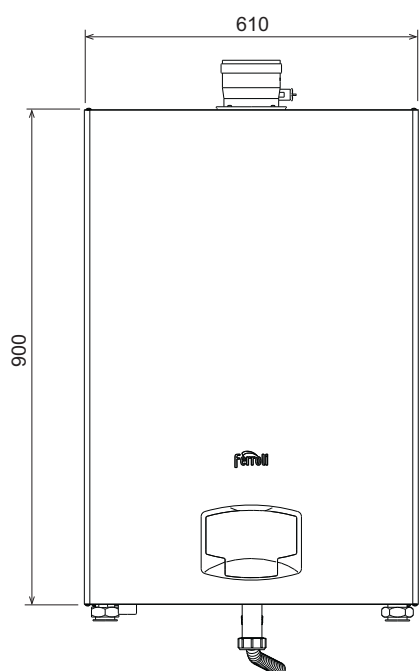
fig. 62- Front view
