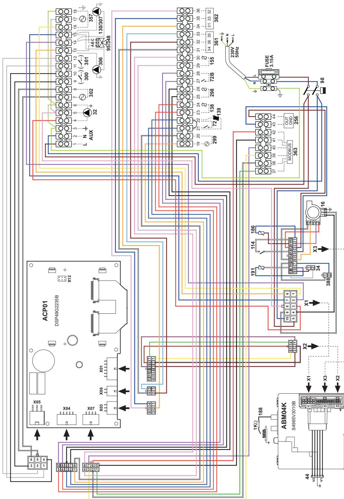
fig. 74- Wiring diagram - models FORCE W 60 and FORCE W 80
