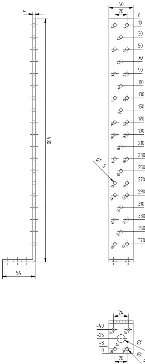
Figure A.80 hold-down 8799 4004 1D
