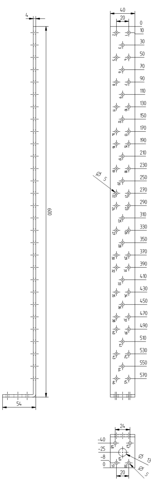
Figure A.84 hold-down 8799 6004 1D
