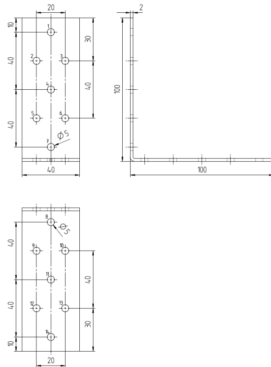
Figure A.18 Angle Bracket 8615
