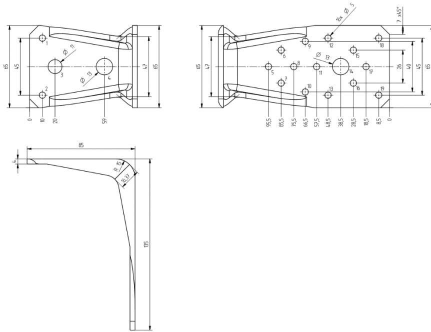
Figure A.5 Angle Bracket 8573 13135 1
