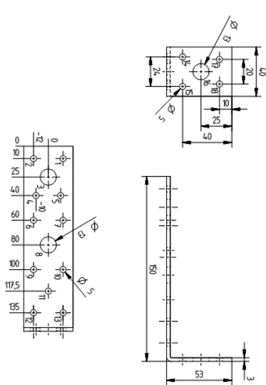
Figure A.63 hold-down 8795 1603 1
