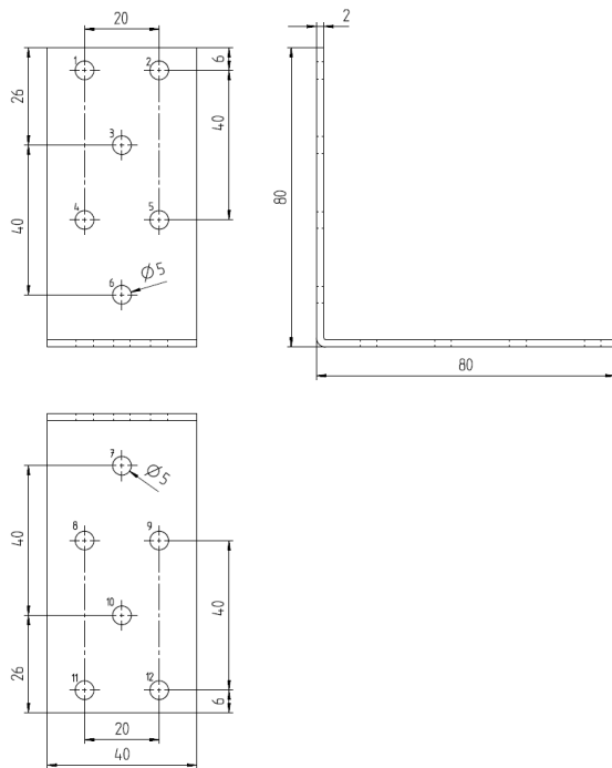
Figure A.17 Angle Bracket 8614
