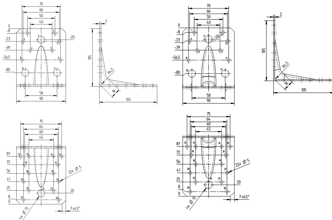
Figure A.41 Angle Bracket 8633 FH
