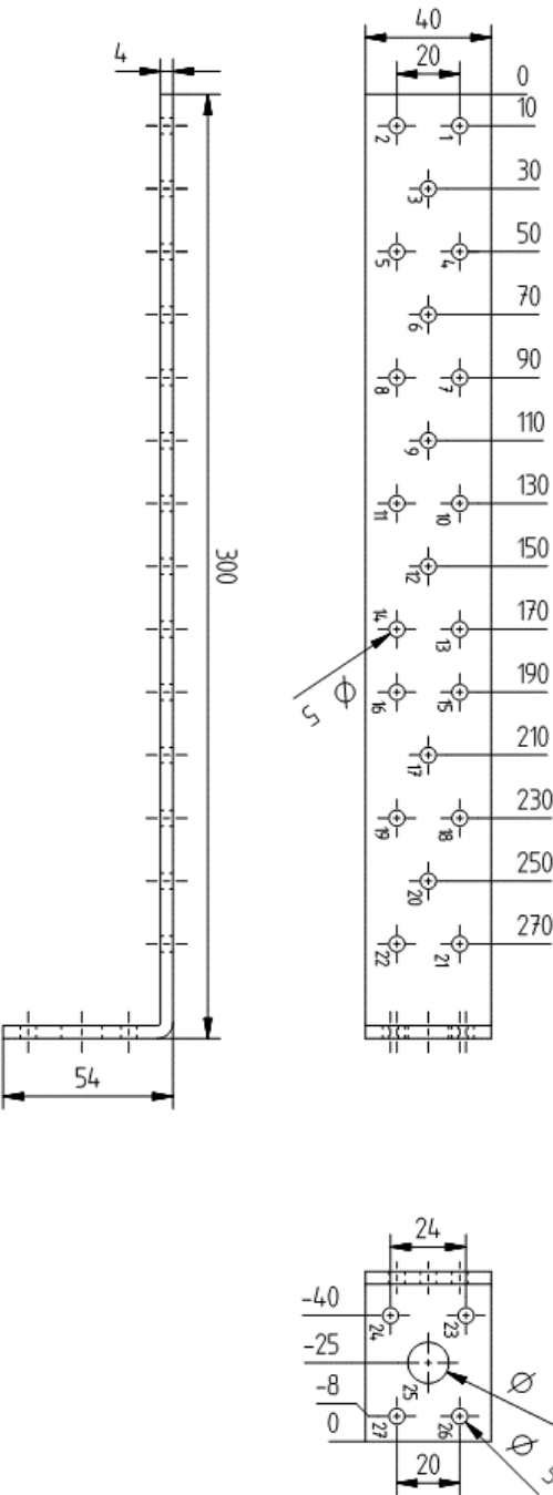
Figure A.78 hold-down 8799 3004 1D
