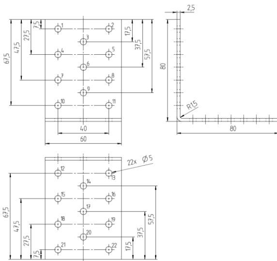
Figure A.49 Angle Bracket 8640
