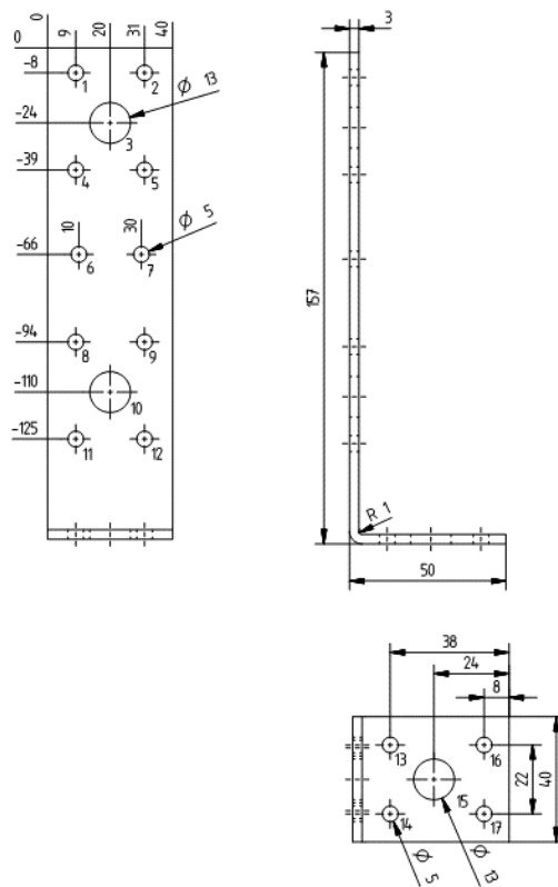
Figure A.64 hold-down 8795 1603 1FH
