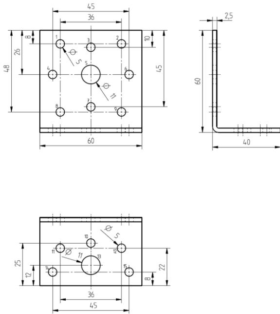
Figure A.15 Angle Bracket 8612
