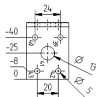
Figure A.82 hold-down 8799 5004 1D
