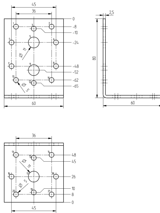
Figure A.16 Angle Bracket 8613
