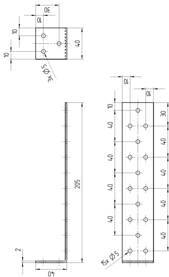
Figure A.57 hold-down 8791
