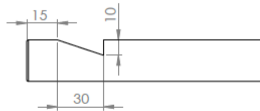
Hangbar detail
