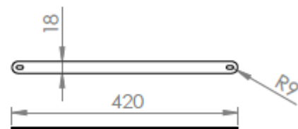
Small reinforcement
