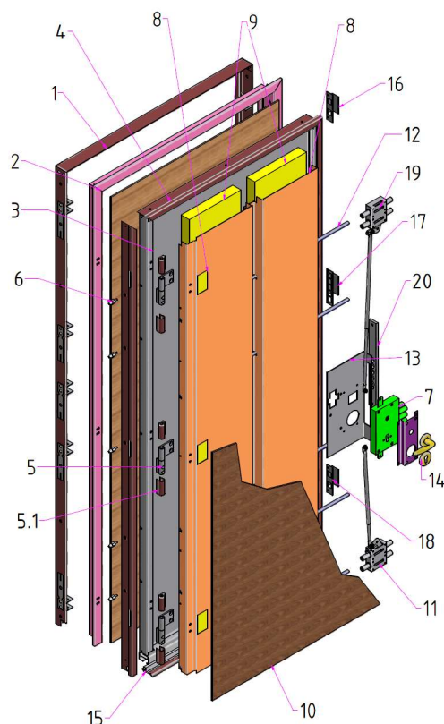
ESPLOSO EXPLODED VIEW
