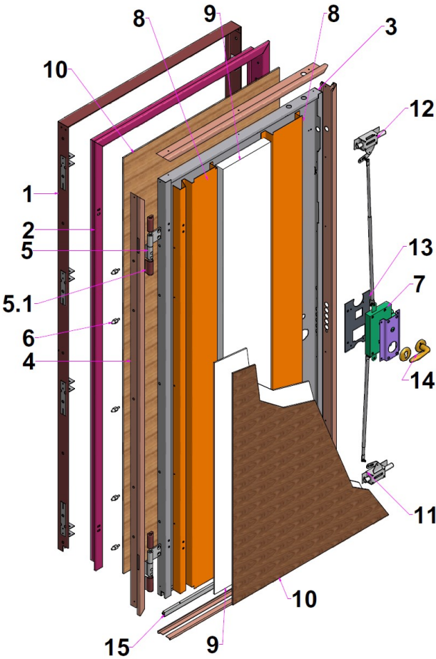
ESPLOSO EXPLODED VIEW
