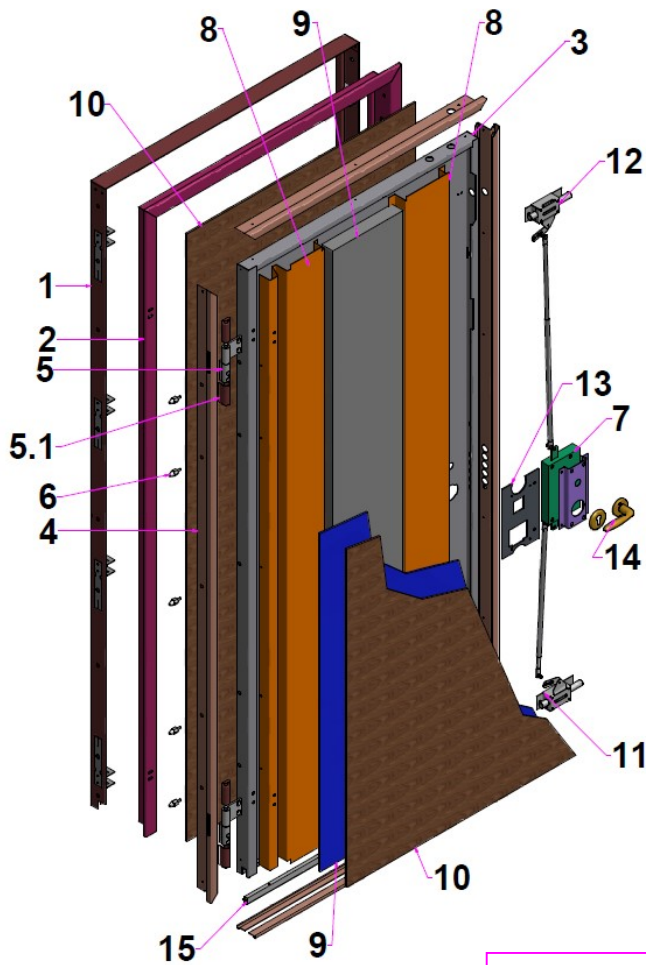
ESPLOSO EXPLODED VIEW
