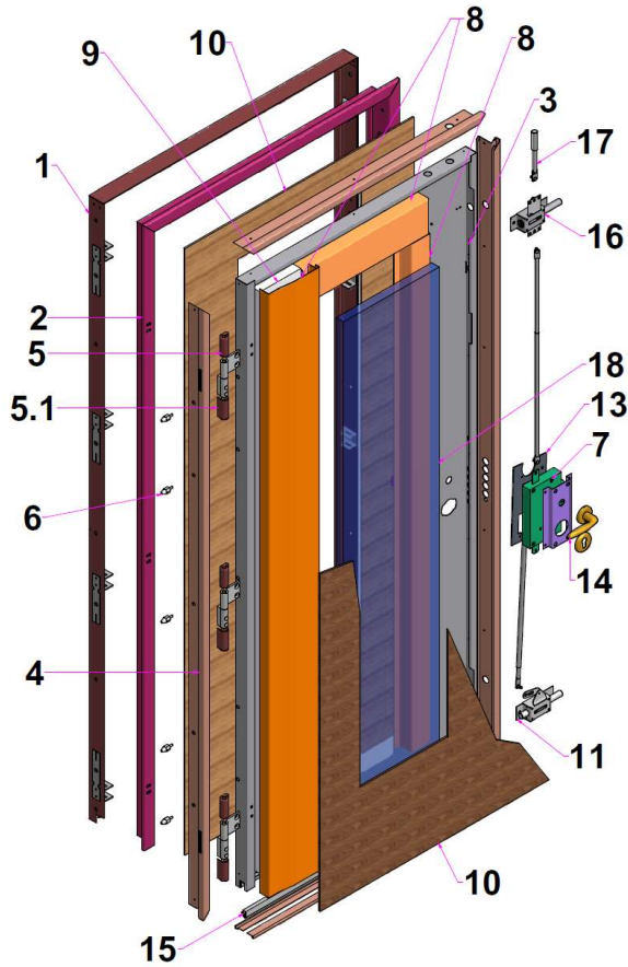
ESPLOSO EXPLODED VIEW
