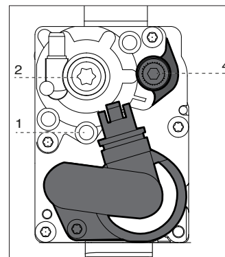
Valvola gas 8205
