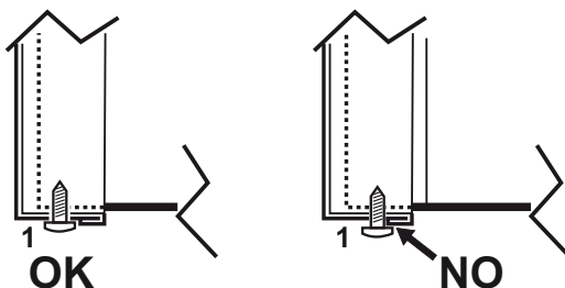
fig. 31- Correct position of front panel
