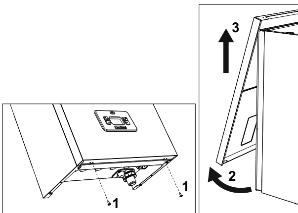
fig. 30- Front panel opening
