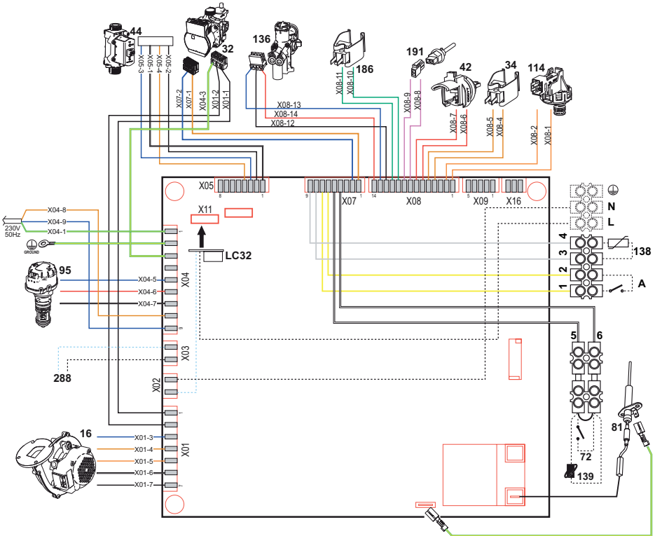
fig. 40- Wiring diagram
