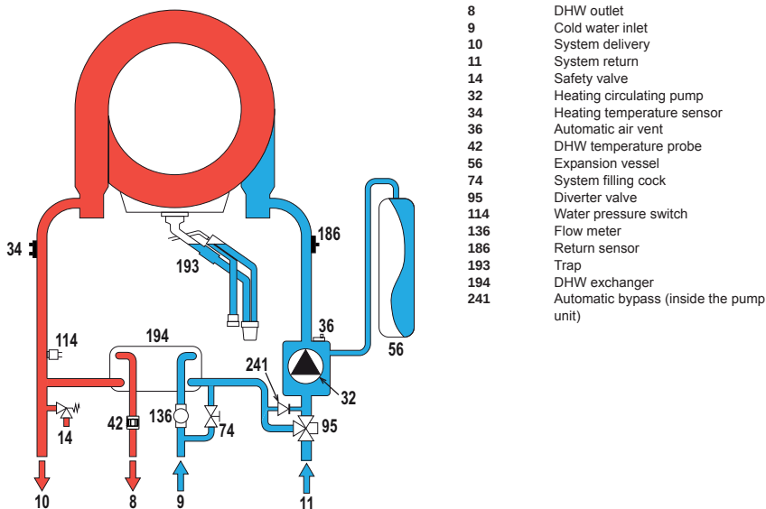
fig. 37- Hydraulic circuit
