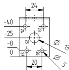
Figure A.67 hold-down 8795 3002 1D
