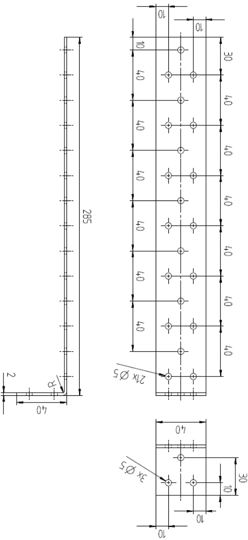
Figure A.59 hold-down 8792
