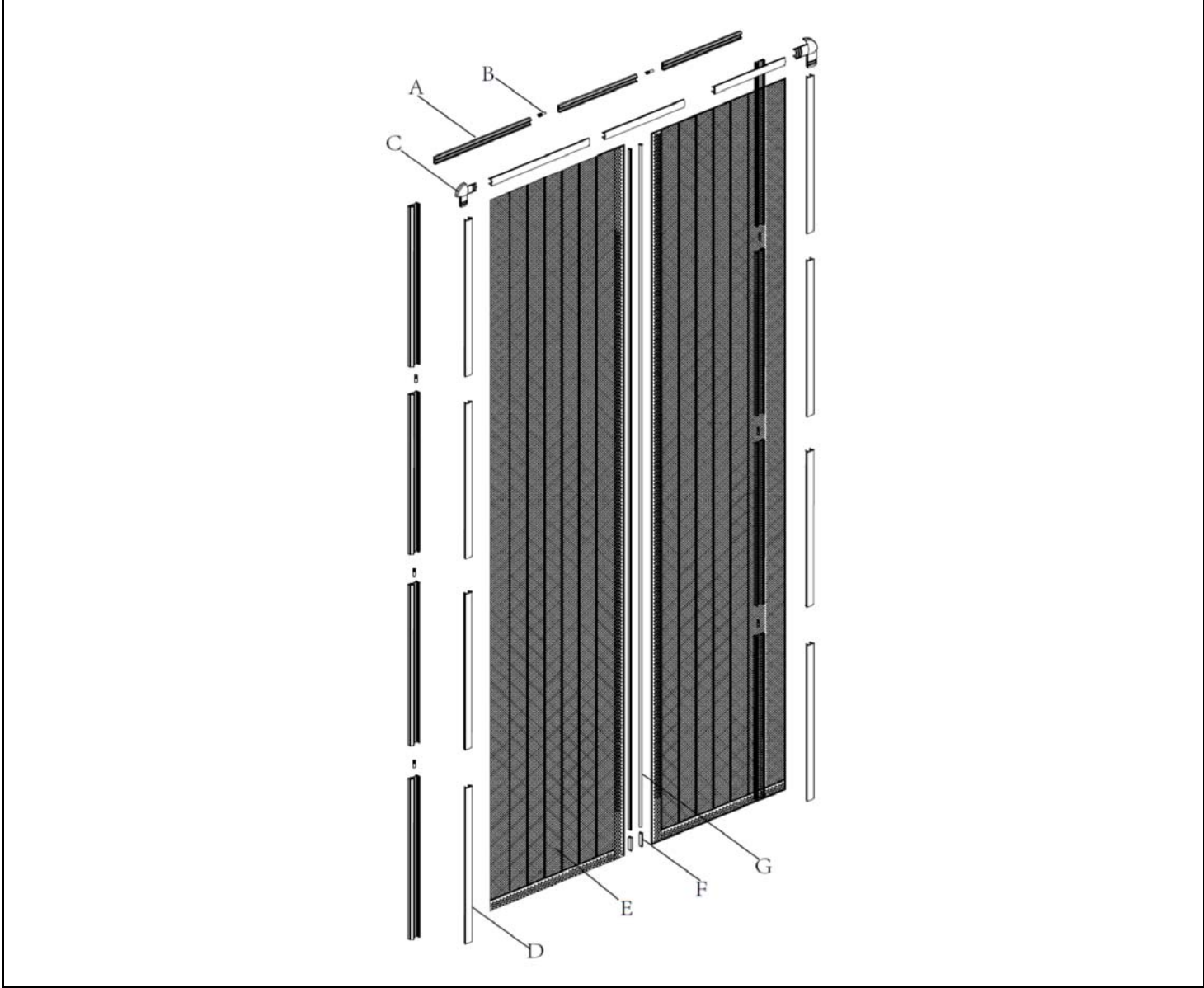
Explosion Drawing
