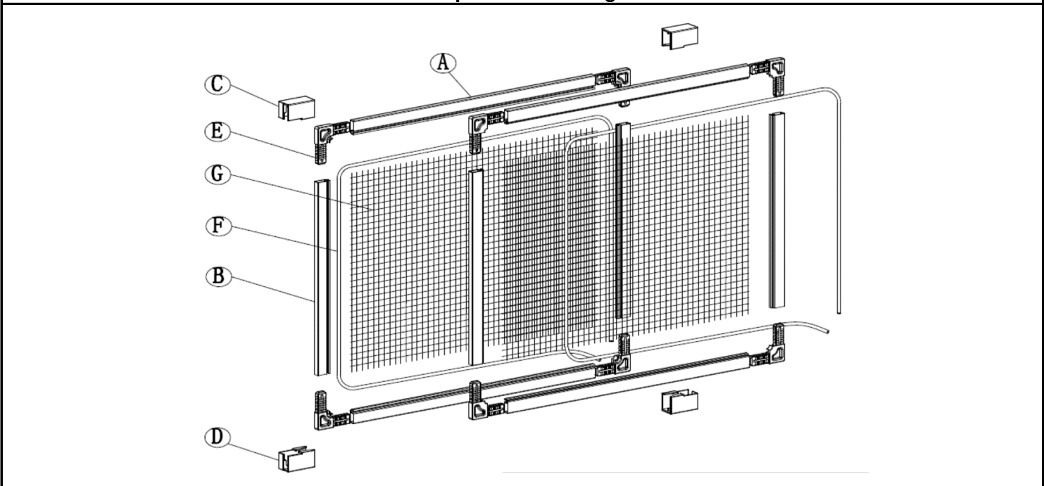
Explosion Drawing
