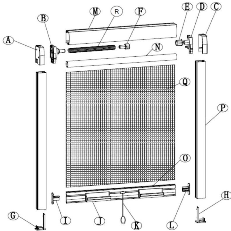
Explosion Drawing
