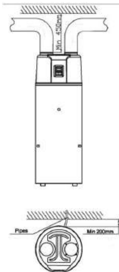
HTW-AT-V200MR290A / HTW-AT-V300MR290A
