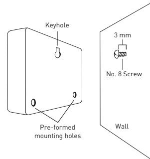
Figure 2: Hang timer on screw using keyhole
