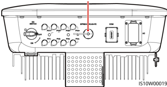
Puerto del Smart Dongle (GPRS/4G/WLAN-FE)
