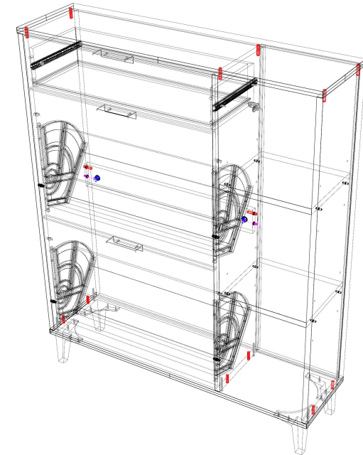
ZAPATERO 2/T+1C K-305 1108x901x245
