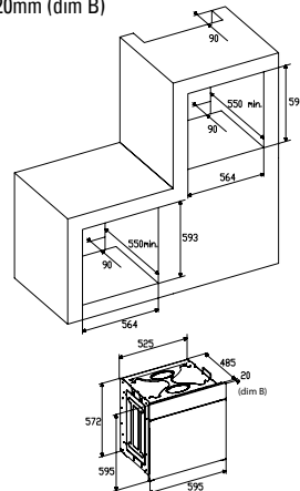
BUILT IN DIMENSION FOR OVEN WITH DOOR THICKNESS OF 20mm (dim B)
