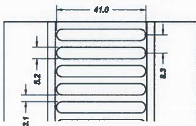
Figure 16 – Accessoire de ventilation F 109
