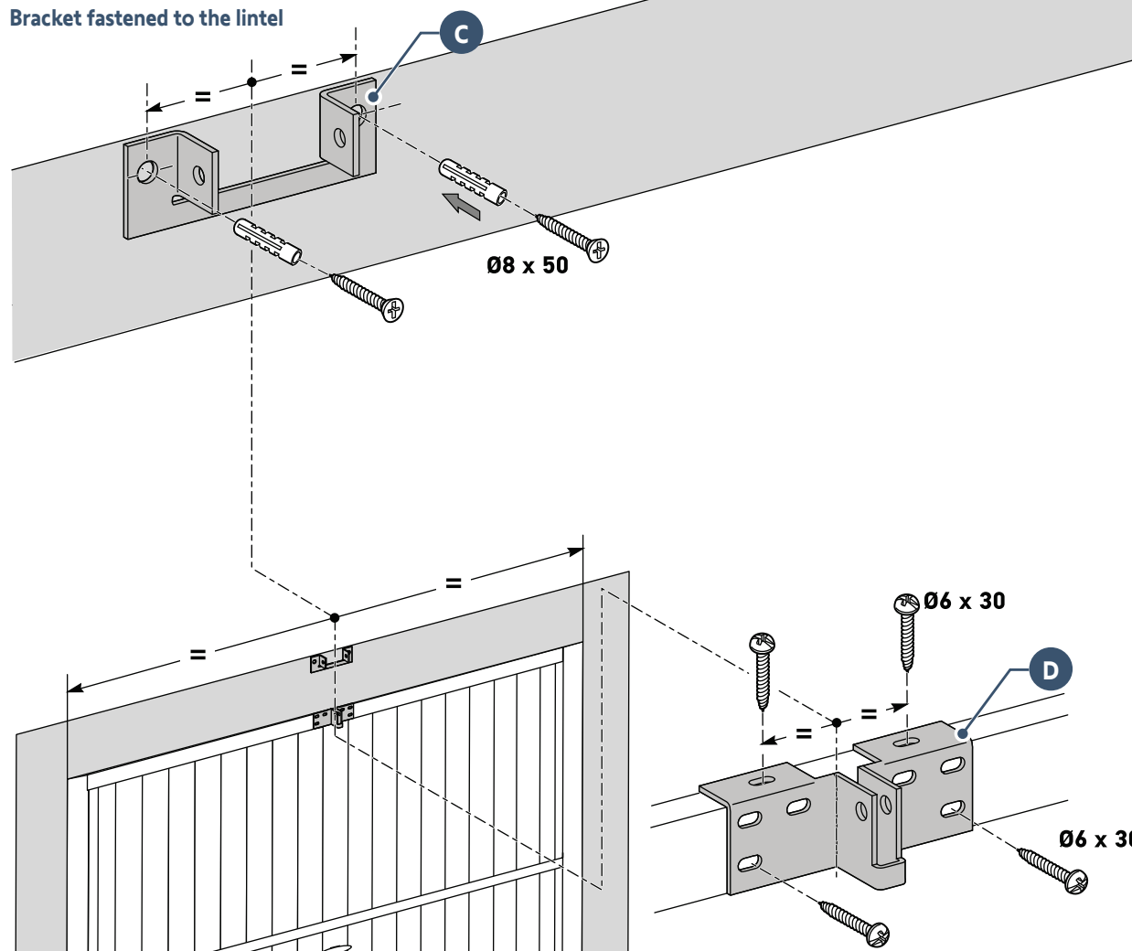
Bracket fastened to the lintel
