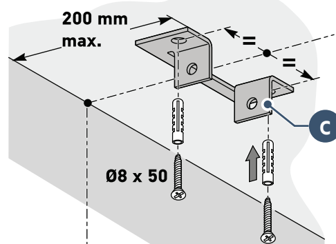
Bracket fastened to the ceiling
