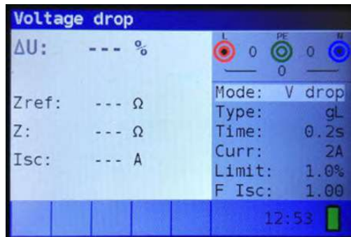
Figura 5 378: Voltage drop measurement menu
