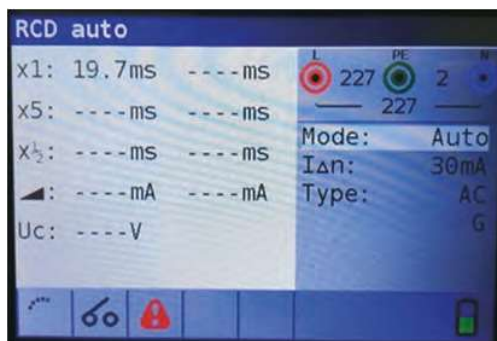
Figure 4 19: Step 1 RCD autotest results
