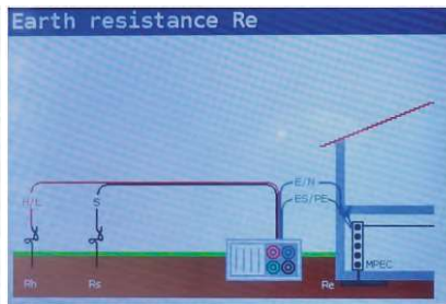
Figure 4 37: 3 wire connection diagram
