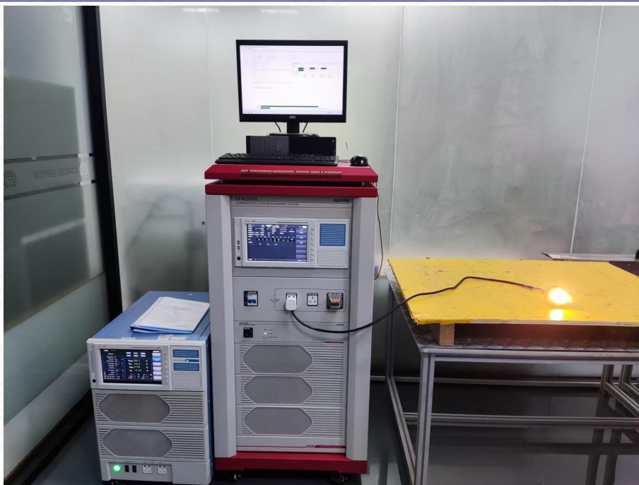
Figure 5: Harmonic & Flicker Test Setup
