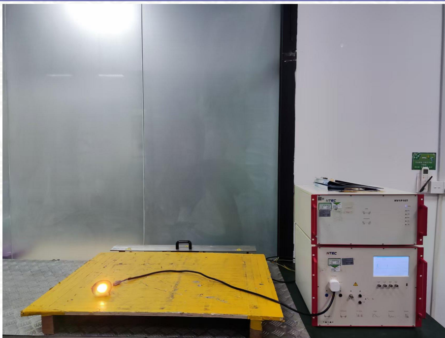
Figure 7: SURGE、DIP&EFT Test Setup
