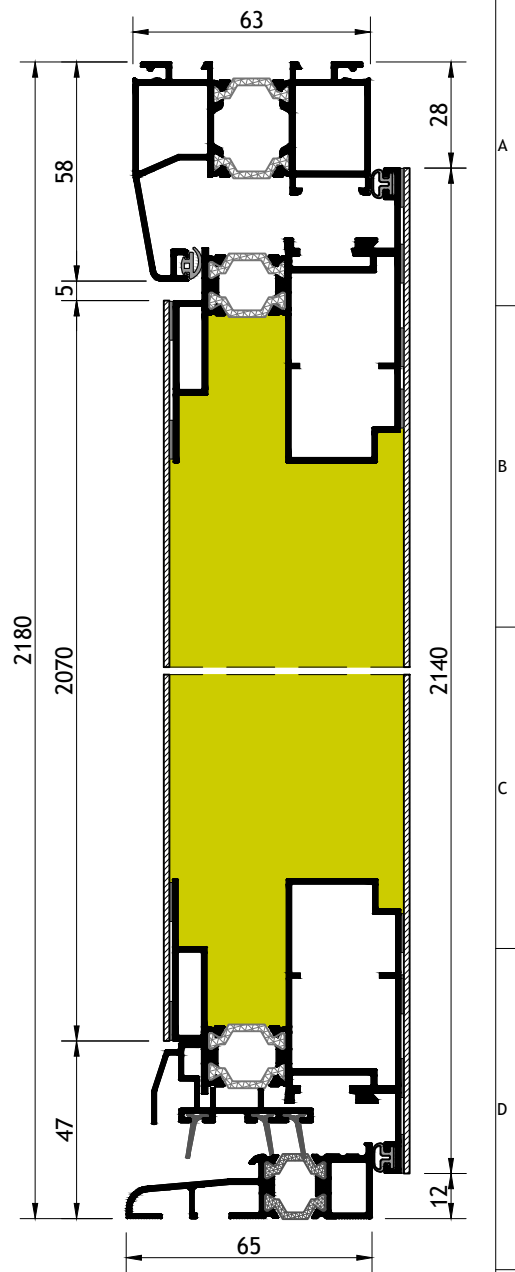
Section B-B
