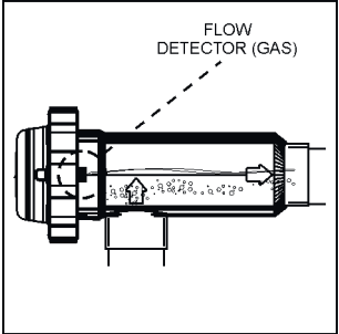
Fig. 6 ALLOWABLE installation
