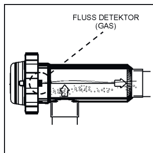
Abb. 6 ERALUBTE Installation
