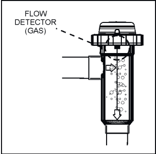
Fig. 5 RECOMMENDED Installation
