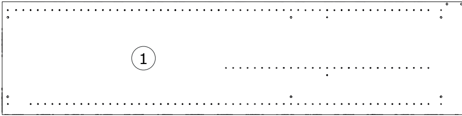
FI10269 2050x500x16mm
