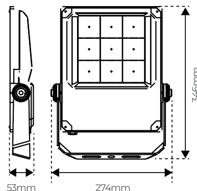
Product Drawing
