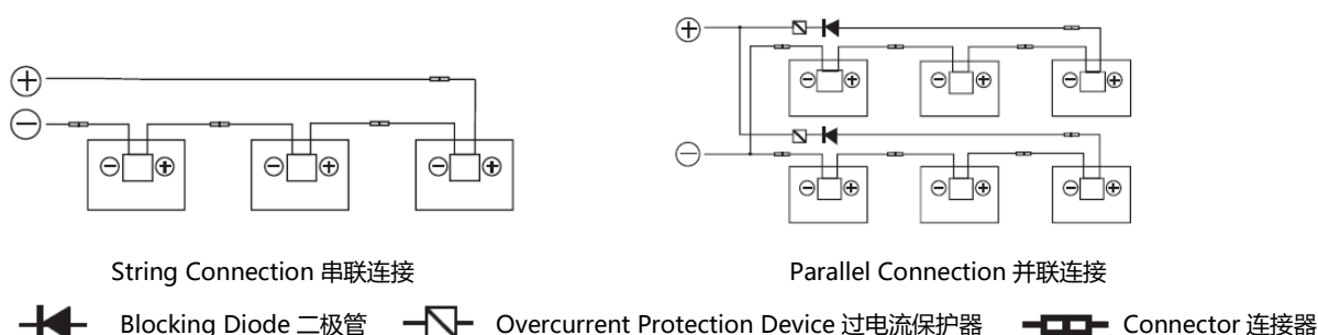
Fig. 5-3 Module connection method
