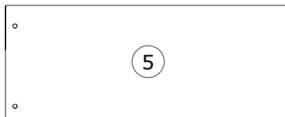
PI08144 1017x404x16mm
