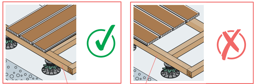
Aluminium joist
