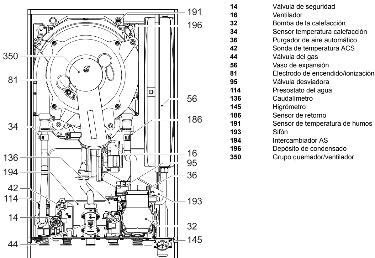
fig. 40- Vista general
