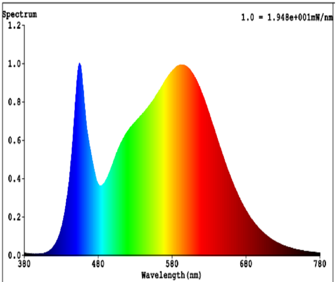
Spectral Distribution
