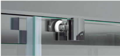
Upper bearing with double sliding system and lower bearing with simple system / Rodamiento superior con sistema doble / Rolamento superior com sistema duplo
