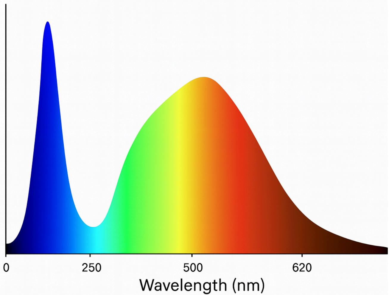
Spectral Power Distribution in the range 250 nm to 800 nm, at full-load
