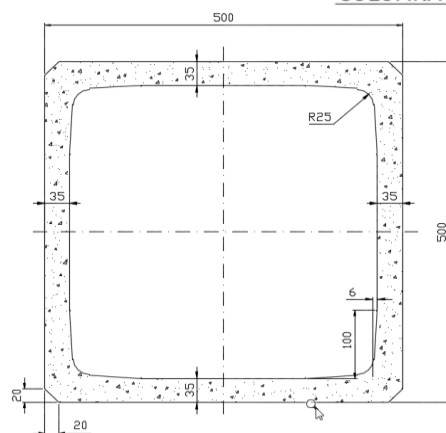
2 COLUMNAS 500x500x200
