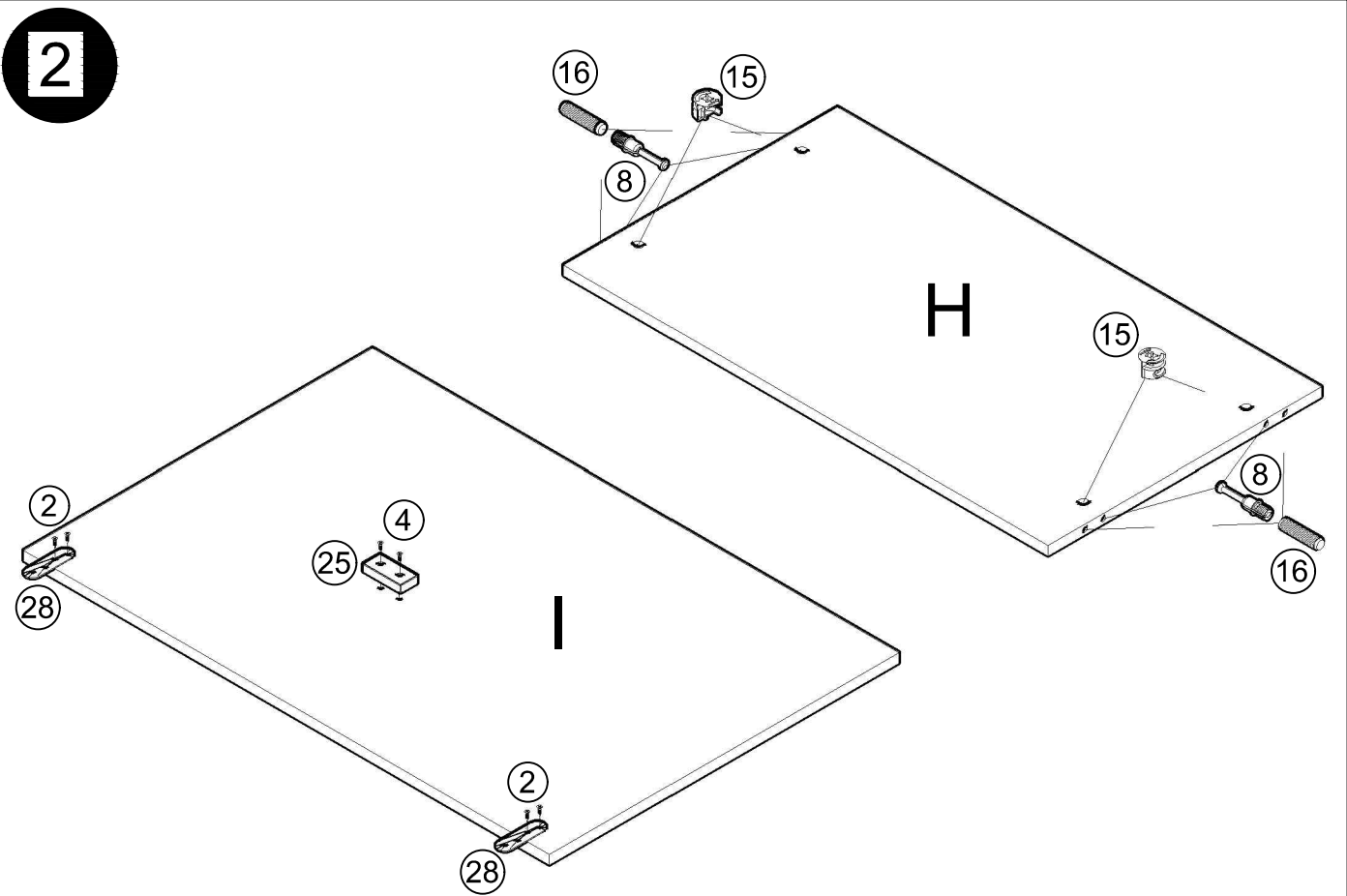
MESA EXTENSIBLE "BASS" 140x90 cm
