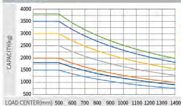
Load curve
